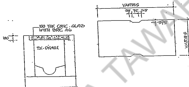
WALKWAY - CONCRETE SLAB
