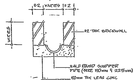
HALF ROUND CULVERT
