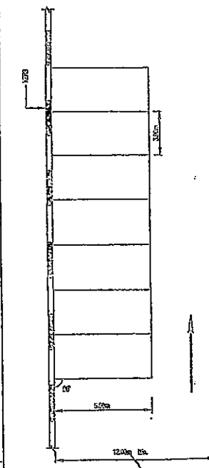
TYPE 1. DETAILS OF PARKING SPACES FOR LIGHT VEHICLES
