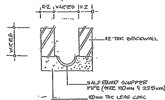
HALF ROUND CULVERT
